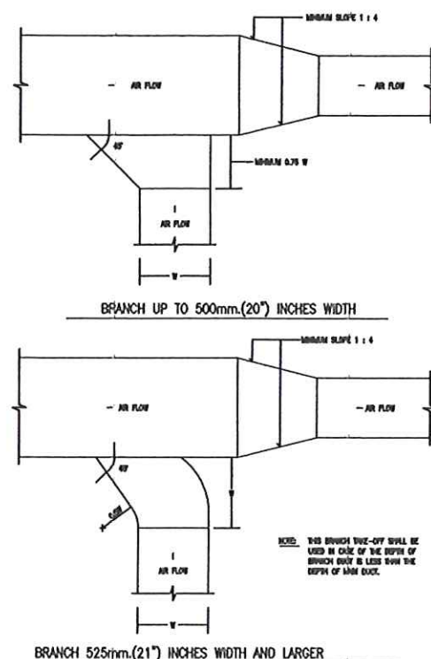
RETURN AND EXHAUST AIR DUCT BRANCH TAKE-OFF
